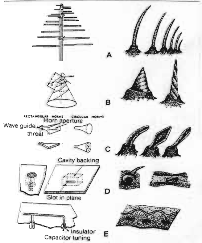
Comparison of insect dielectric and man-made metal antennae. (A) Log periodic spacing; (B) Conical spiral type; (C) Horn and lens types; (D) Cavity types; (E) Loop types.
